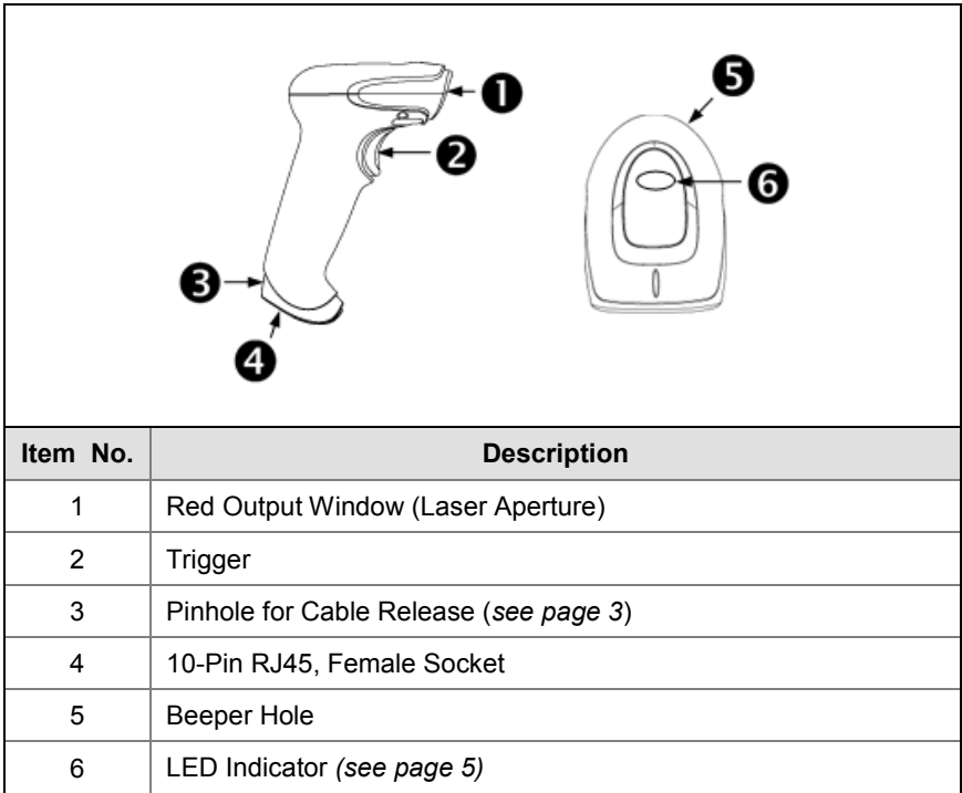
Figure 1. Scanner Components
